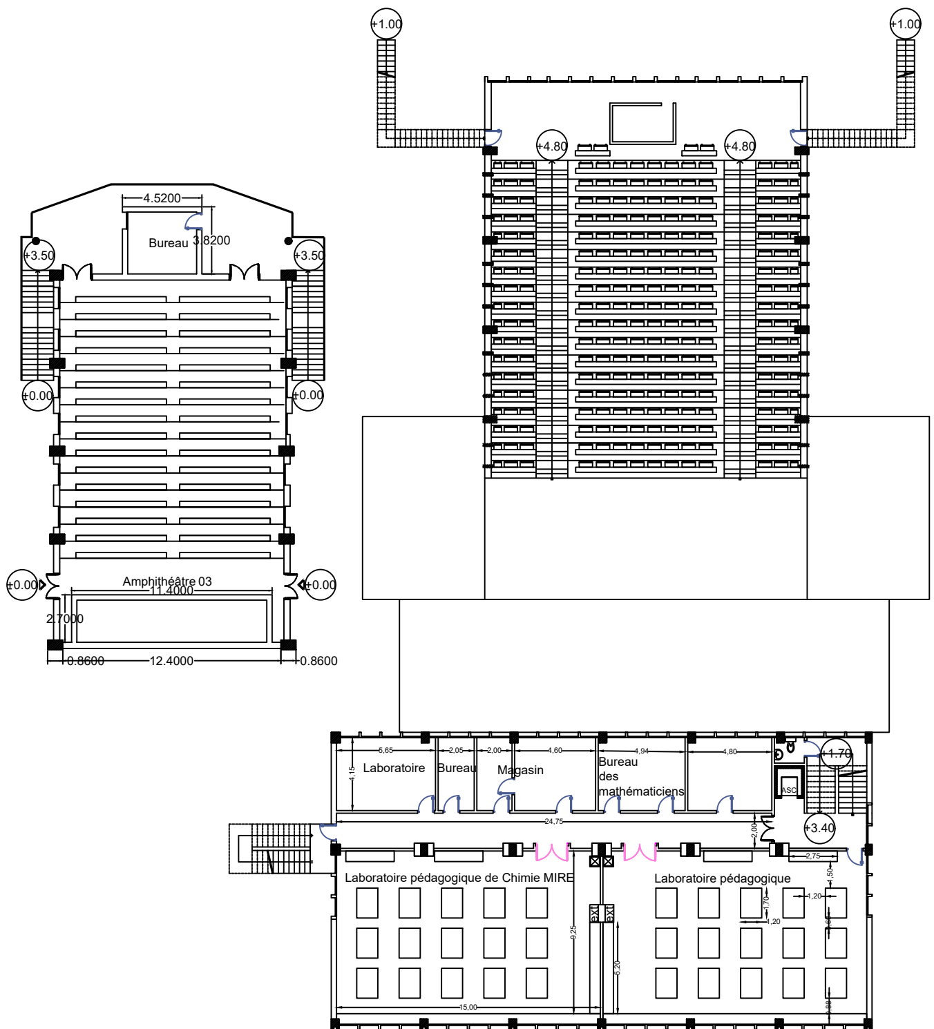
PLAN 1ER ETAGE Ech = 1/200
